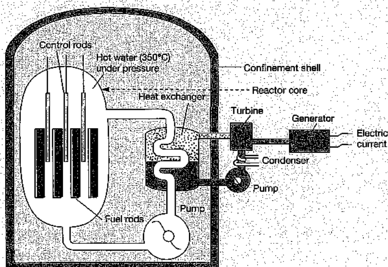
A nuclear power plant
